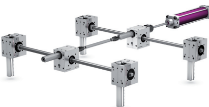
Levage 4 points
